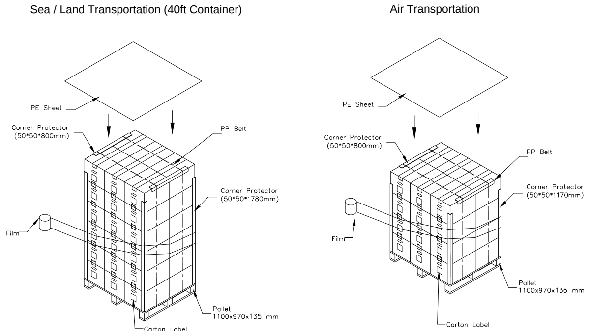
Figure. 9-2 Packing method
